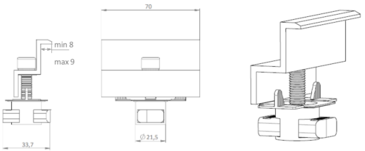
Figure 12 : Étrier final
