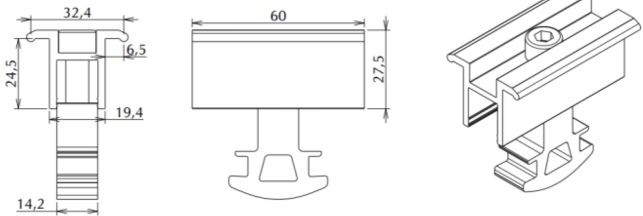
Figure 14 : Étrier universel FATH
